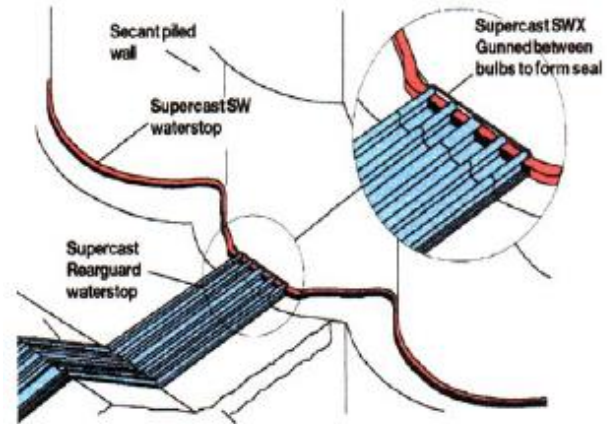
Supercast SW, Supercast SWX and Supercast Rearguard waterstops at secant pile wall and floor slab junction
