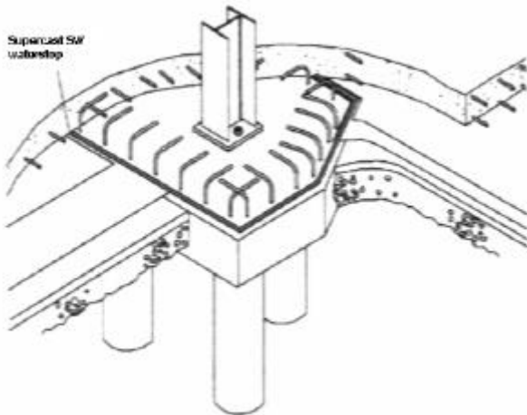
Pile cap detail using Supercast SW waterstop
